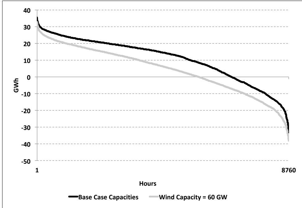
Figure 3: Net Load Duration Curves, 2030 Forecast Scenario and Base Case Capacity.
