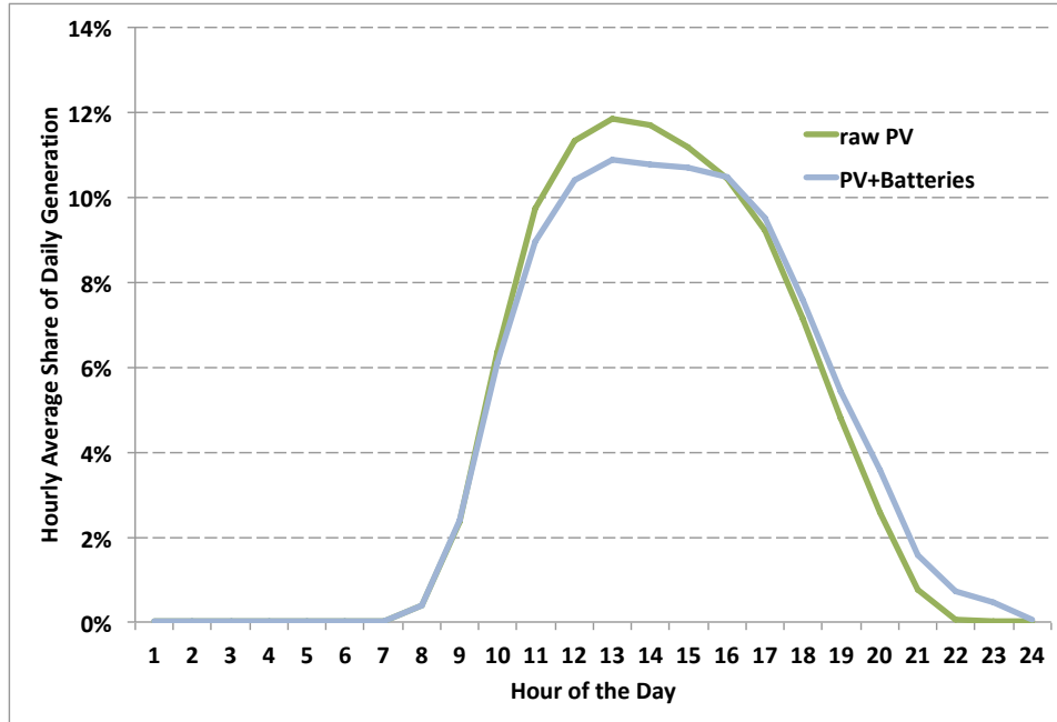
Figure 5: The Average Hourly Generation Profile of Solar PV, Gross and Net of Battery Use, 2030 Forecast Scenario.
