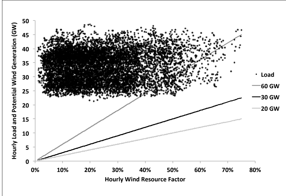
Figure 2: The Correspondence Between the Hourly Wind Resource Factor and the Hourly Load, 2030 Forecast Scenario.
