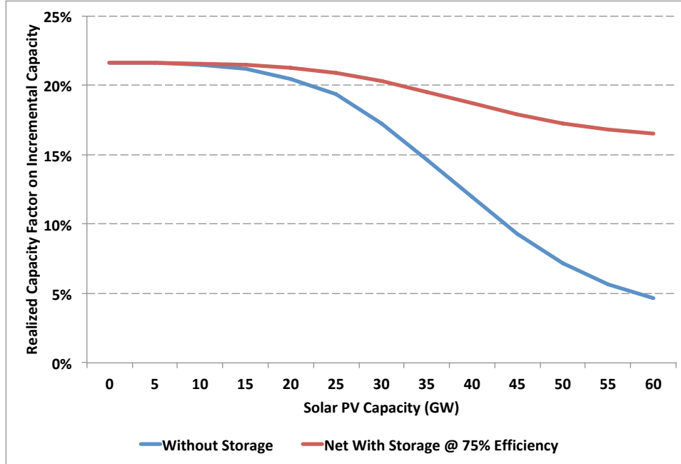
Figure 4: The Declining Capacity Factor for Incremental Solar Capacity, 2030 Forecast Scenario.
